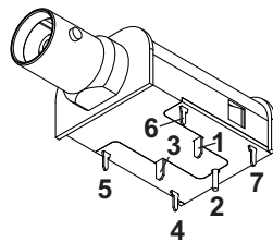
Anschlussplan Connecting diagram Plan de raccordement
