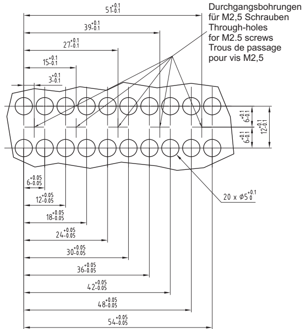
Bohrplan Drilling-scheme Plan de perçage
